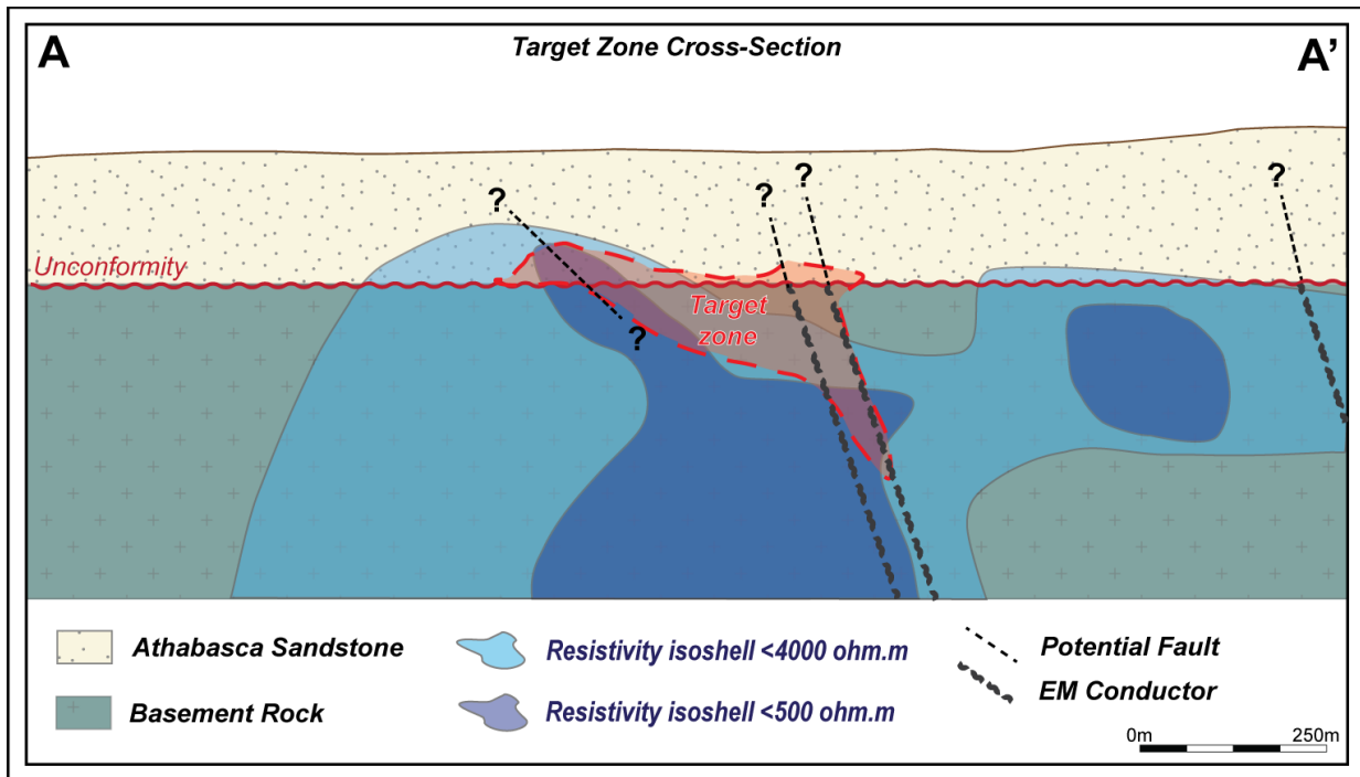
Figure 3. Schematic cross-section A-A' (Figure 2) facing west through the northern conductor trend on the Project, highlighting significant resistivity anomalies coincident with modeled EM conductors.
